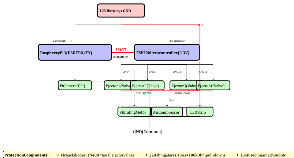
Figure 4.1: Electrical schematic: power distribution, processor connections, actuator outputs, and communication links
